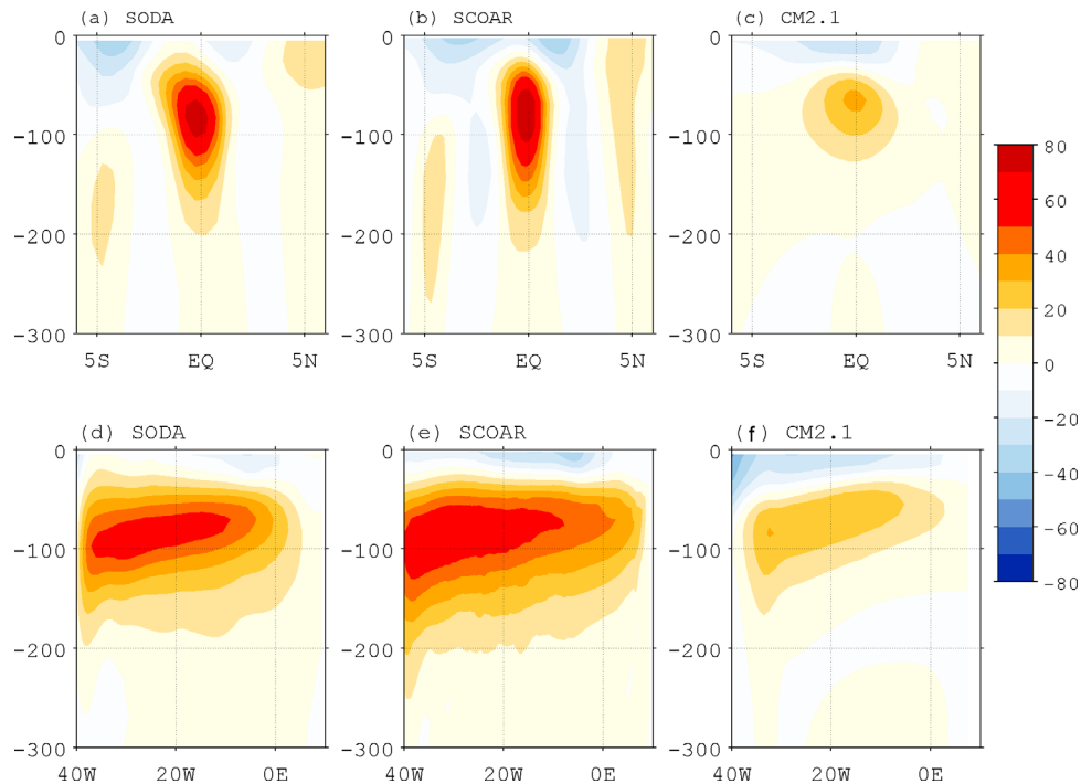
Figure 3. (a–c) Meridional and (d–f) zonal transects of annual mean (1998–2007) zonal current speed ( \text{cm s}^{-1} ) from SODA (Figures 3a and 3d), SCOAR (Figures 3b and 3e), and CM2.1 (Figures 3c and 3f). The zonal currents are averaged 30^{\circ}\text{W} – 10^{\circ}\text{W} for Figures 3a–3c and 1^{\circ}\text{S} – 1^{\circ}\text{N} for Figures 3d–3f. The Equatorial Undercurrent is shown in red shades that flow eastward at a depth of \sim 75 m. The South Equatorial Current is separated into northern and southern branches across the equatorial and flows westward near the surface.
