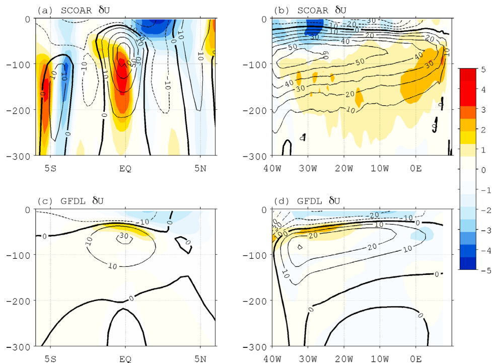
Figure 8. Annual mean (1998–2007) difference ( \delta , shade) in zonal currents ( \text{cm s}^{-1} ) from (a, b) SCOAR and (c, d) CM2.1 averaged over 30^{\circ}\text{W} – 10^{\circ}\text{W} (Figures 8a and 8c) and 1^{\circ}\text{S} – 1^{\circ}\text{N} (Figures 8b and 8d). The present-day climatological values are superimposed in black contours with \text{CI} = 10 \text{ cm s}^{-1} .
