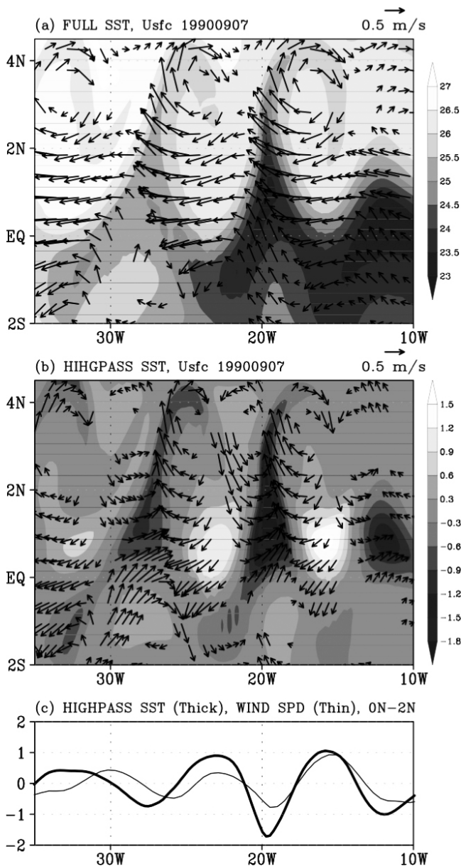
Figure 13. Snapshots from CTL of SST and surface currents on 7 September 1990 showing (a) full fields and (b) zonally high-pass filtered fields ( 10^\circ longitudes). (c) High-pass filtered SST (thick line) and wind speed (thin line) averaged over the equator to 2^\circ\text{N} .
