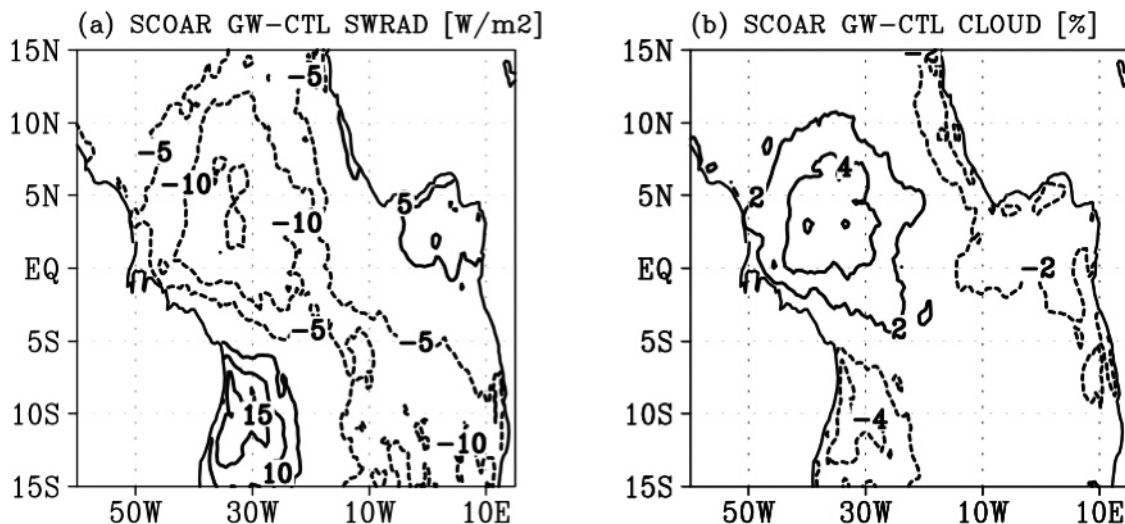
Figure 6. Annual mean changes (GW-CTL) in (a) downward shortwave radiation (SWRAD, W/m 2 , contour interval (CI) = 5 W/m 2 ) and (b) total cloud amount (CLOUD, %, CI = 2%) from SCOAR. Negative values are shown as dashed contours.
