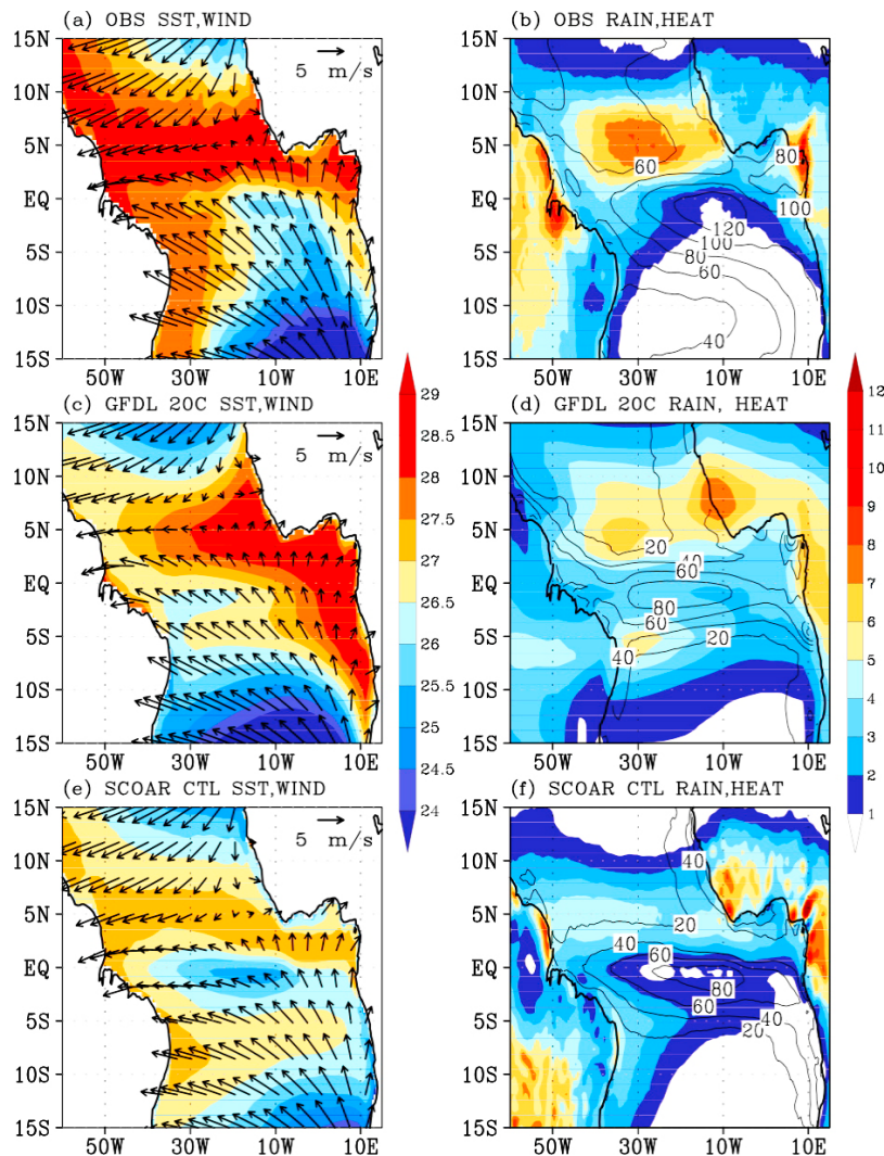
Figure 2. (a, c, e) Annual mean SST ( ^{\circ}\text{C} , color shade) and the 10 m winds and (b, d, f) precipitation ( \text{mm d}^{-1} , color shade) and the surface net heat flux ( \text{N m}^{-2} , black contour with interval 20 \text{ N m}^{-2} ) for observations (NOAA OI SST Analysis and NCEP2 10 m winds, both from 1998 to 2007, the precipitation from TRMM 3B43 product (1998–2007) and the OAFlux from 1998 to 2004, Figures 2a and 2b), CM2.1 20C simulation (1996–2000, Figures 2c and 2d), and SCOAR CTL run (1998–2007, Figures 2e and 2f).
