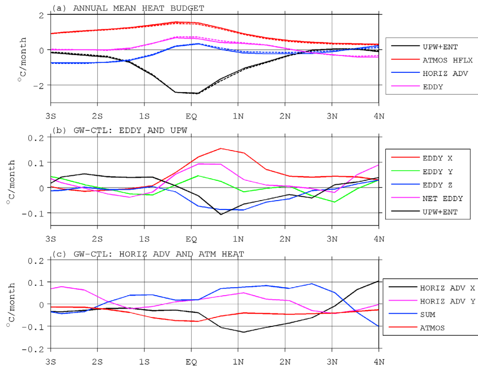
Figure 11. (a) Zonally averaged ( 30^{\circ}\text{W} – 10^{\circ}\text{W} ) annual mean heat budget ( ^{\circ}\text{C month}^{-1} , 1998–2007) as a function of latitude. Solid lines are for CTL and dashed lines are for GW. Upwelling and entrainment (black), atmospheric heat flux into the ocean (red), mean horizontal advection of temperature (blue), and three-dimensional eddy temperature advection (magenta). (b) Difference (GW-CTL) for upwelling and entrainment (black), net eddy heat flux (magenta), zonal eddy heat flux (red), meridional eddy heat flux (green), and vertical eddy heat flux (blue). (c) Difference (GW-CTL) for atmospheric heat flux (red), net horizontal advection (blue), and horizontal advection with zonal (black) and meridional (magenta) component.
