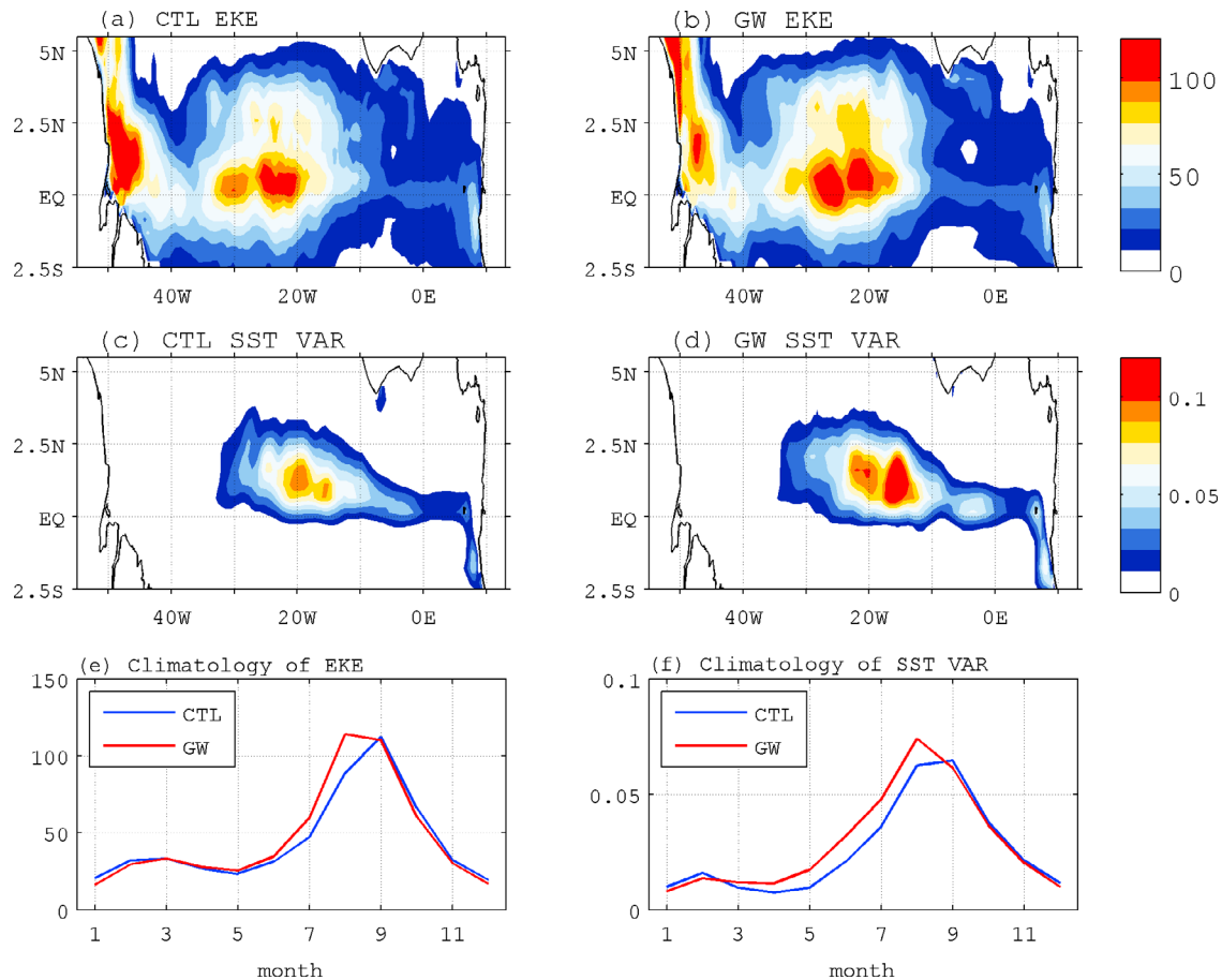
Figure 10. June–August averaged eddy kinetic energy (EKE, \text{cm}^2 \text{s}^{-2} ) defined as \text{EKE} = 1/2 (u'^2 + v'^2) , where ' denotes 20–40 day band-pass filtering for (a) CTL and (b) GW from 1998 to 2007. (c, d) As in Figures 10a and 10b except for the variance of 20–40 day filtered SST. Annual cycle of (e) EKE and (f) SST variance as a function of calendar month for CTL (blue) and GW (red).
