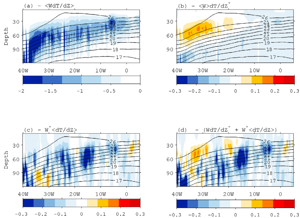
Figure 7. Decomposition of the 10 year annual mean vertical temperature advection ( ^{\circ}\text{C month}^{-1} ) in SCOAR averaged over 3^{\circ}\text{S} – 3^{\circ}\text{N} based on monthly climatology for (a) -\langle w \rangle \langle T_z \rangle , (b) -\langle w \rangle T_z^* , (c) -w^* \langle T_z \rangle , and (d) the sum of Figures 7b and 7c, -(\langle w \rangle T_z^* + w^* \langle T_z \rangle) . Ocean temperature in CTL run is superimposed in black contours with contour interval of 1^{\circ}\text{C} . Note the different scales between Figure 7a and Figures 7b–7d.
