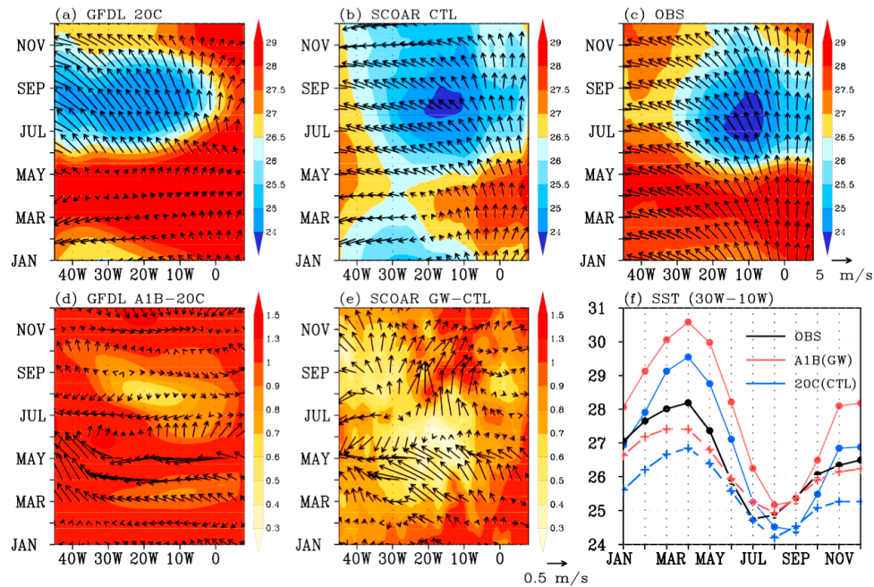
Figure 4. Seasonal cycle of equatorial cold tongue ( 1^{\circ}\text{S} – 1^{\circ}\text{N} ) of (a) CM2.1 20C, (b) SCOAR CTL, (c) OBS, (d) CM2.1 A1B-20C, and (e) SCOAR GW-CTL. (f) The annual cycles of SST ( 30^{\circ}\text{W} – 10^{\circ}\text{W} , 1^{\circ}\text{S} – 1^{\circ}\text{N} ) in observations (black), CM2.1 20C (blue solid line with circles), CM2.1 A1B (red solid line with circles), SCOAR CTL (blue dashed line with crosses), and SCOAR GW (red dashed line with crosses).
