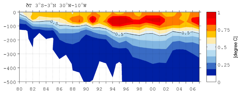
Figure 1. Evolution of annual mean temperature over the equatorial cold tongue ( 3^{\circ}\text{S} – 3^{\circ}\text{N} , 30^{\circ}\text{W} – 10^{\circ}\text{W} ) from 1980 to 2007. The black contour denotes the increase of temperature by 0.5^{\circ}\text{C} .
