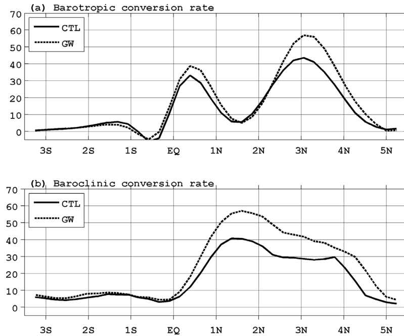
Figure 9. (a) Barotropic conversion ( 10^{-6} \text{ kg m}^{-1} \text{ s}^{-3} ), -\rho_o \bar{u}' \cdot (\bar{u}' \cdot \nabla \bar{U}) for CTL (solid line) and GW (dashed line), averaged for upper 100 m over 30^\circ\text{W} – 10^\circ\text{W} for June–August of 10 years. (b) Same as Figure 9a except for baroclinic conversion, -g\rho'w' . Calculations based on annual mean show similar results.
