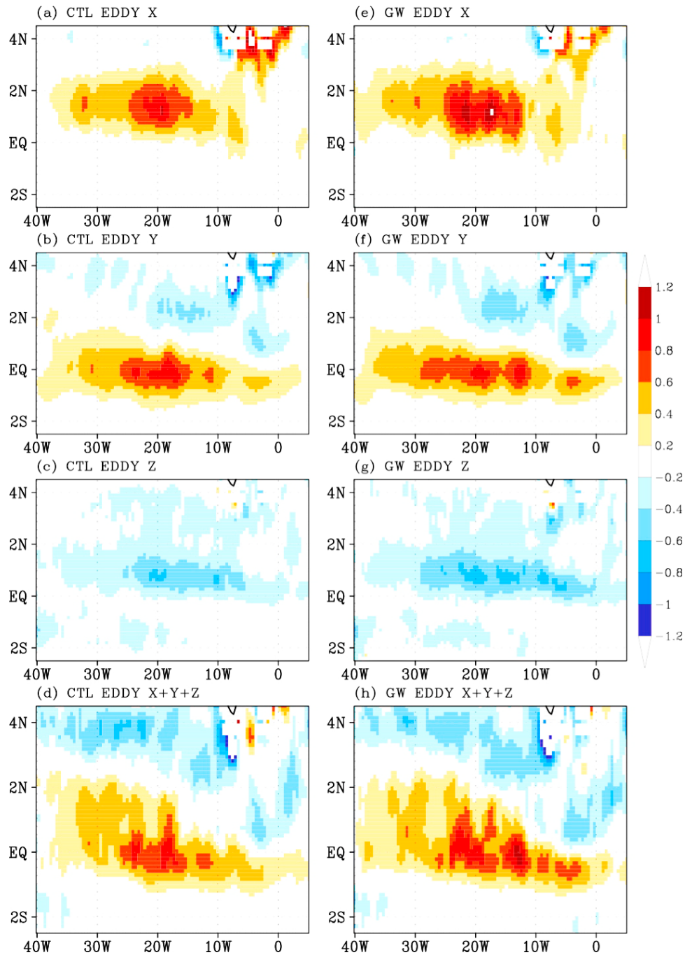
Figure 12. Each component of the annual mean eddy temperature advections ( ^{\circ}\text{C month}^{-1} ) in (a–d) CTL and (e–h) GW averaged from 1998 to 2007: zonal (Figures 12a and 12e), meridional (Figures 12b and 12f), vertical (Figures 12c and 12g), and the sum (Figures 12d and 12h). The contour intervals are 0.2^{\circ}\text{C month}^{-1} .
